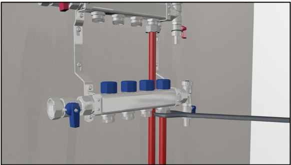
Return the first pipe run to the manifold.
